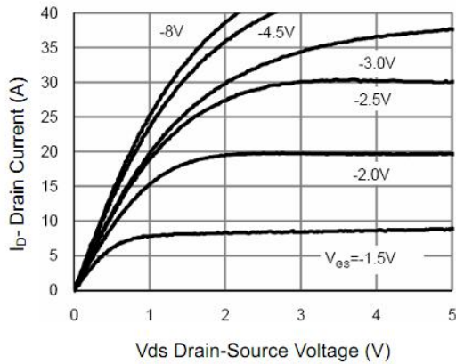
Figure 1: Output Characteristics
