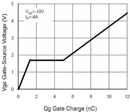
Figure 5: Gate-Charge Characteristics
