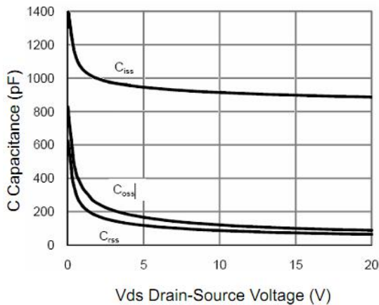
Figure 3: Capacitance
